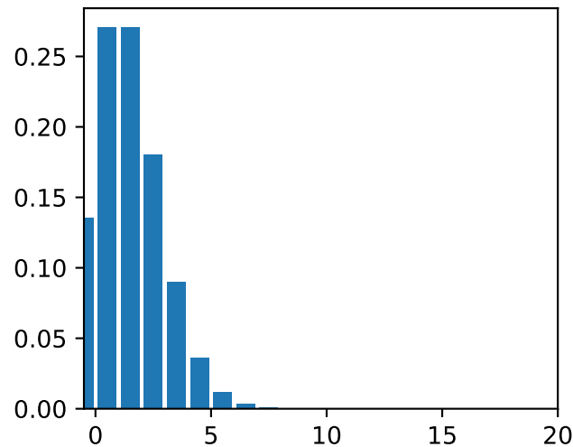
Coherent state
