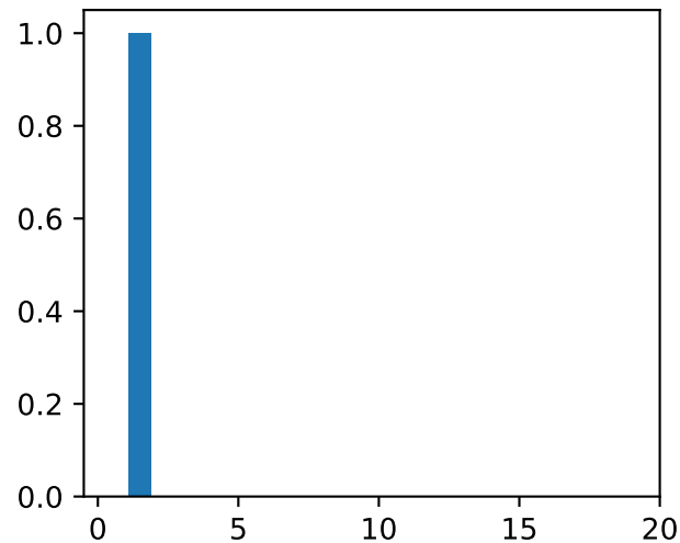
Fock state
